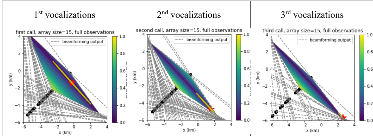
Figure 11. Localization result using the grid search method from Abadi et al. (2015, 2017) for a 15-element subarray for the vocalizations shown in Figure 10
