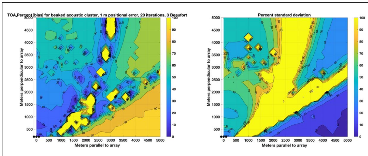
Figure 8. Relative bias (left) and variance (right) expressed as a percentage for 20 iterations of a simulated beaked whale signal for the three-element time-of-arrival (TOA) localization geometry, incorporating 1-m uncertainty in hydrophone position Small black circles indicate hydrophone positions. White areas indicate locations with no valid solution.
