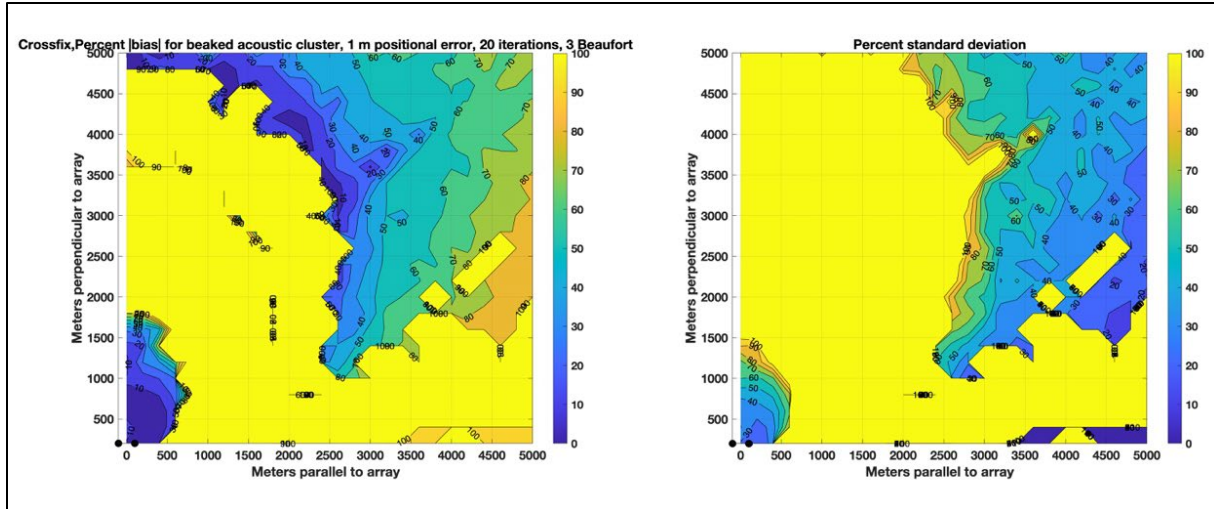
Figure 9. Relative bias (left) and variance (right) expressed as a percentage for 20 iterations of a simulated beaked whale signal using the cross-fixing localization algorithm, incorporating 1-m uncertainty in hydrophone position and 10^\circ uncertainty in subarray heading
