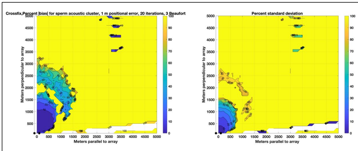
Figure 5. Relative bias (left) and variance (right) expressed as a percentage for 20 iterations of a sperm whale scenario using the four-element cross-fixing localization algorithm, incorporating 1-m uncertainty in hydrophone position and 10° uncertainty in subarray heading Small black circles indicate hydrophone positions. White areas indicate locations with no valid solution.
