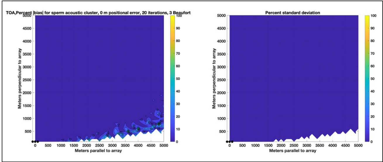
Figure 2. Relative bias (left) and variance (right) expressed as a percentage, for 20 iterations of sperm whale scenario for the three-element time-of-arrival (TOA) localization geometry with no hydrophone localization uncertainty
