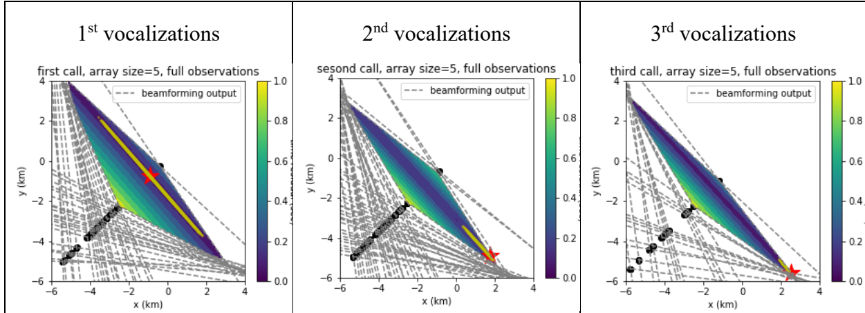
Figure 12. Localization result using the grid search method from Abadi et al. (2015, 2017) for a 5-element subarray for the vocalizations shown in Figure 10
