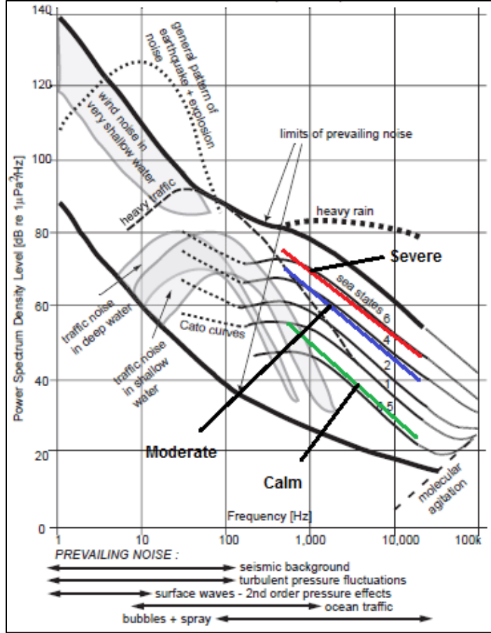
Figure 1. The noise Wenz curves included in the simulation, characterized by sea state (Beaufort force minus 1) and shipping level Based on work by Wenz (1962).
