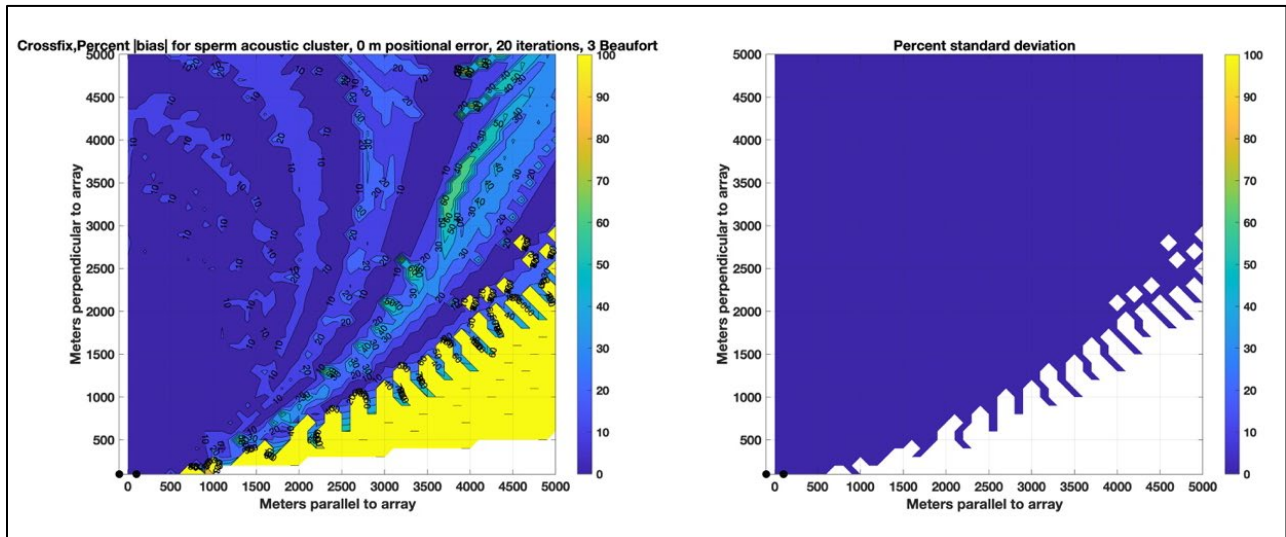
Figure 3. Relative bias (left) and variance (right) expressed as a percentage, for 20 iterations of a sperm whale scenario using the four-element cross-fixing localization algorithm, with no hydrophone localization uncertainty
